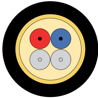
MiDia® Breeze ZS Fibre Optic Cable Cross-Section (2-4 Fibre)
