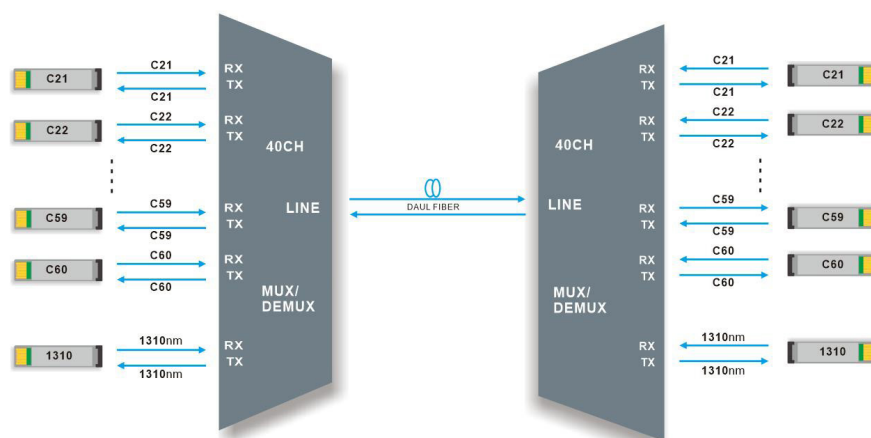
Figure 2. 40CH DWDM MUX DEMUX Dual fiber transmission
