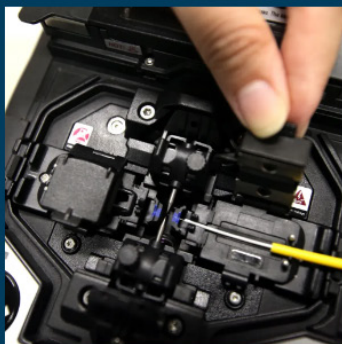
FTTx Access & Fiber Optic Cabling
