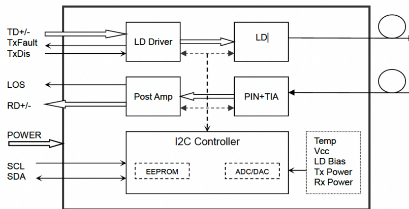
Transceiver functional diagram
