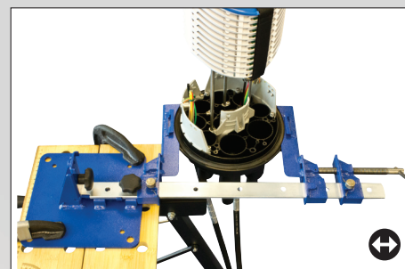
Horizontal Mounting
