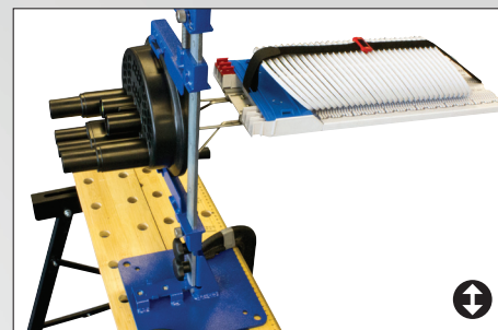
Vertical Mounting
