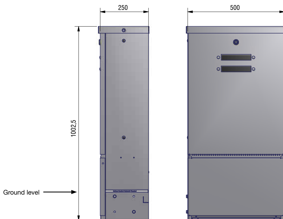
Type SCC 500-250 “Hammar” marking system
