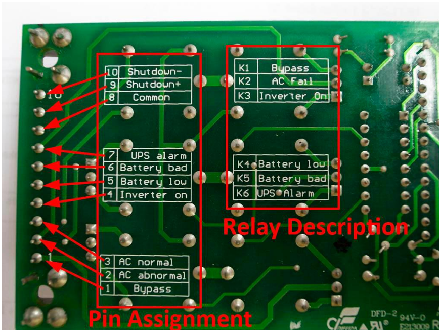
Bottom view
